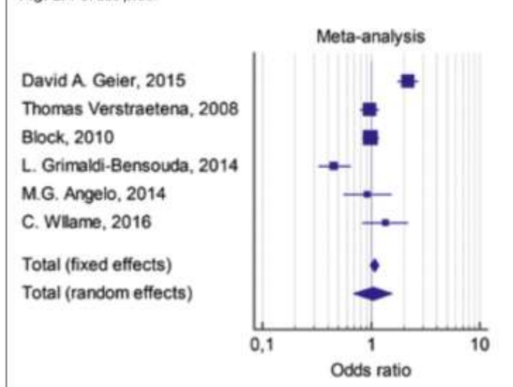
Fig. 2. Forest plot.
